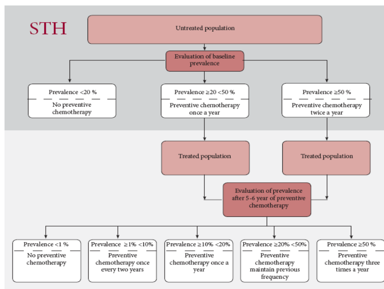
Decision trees
